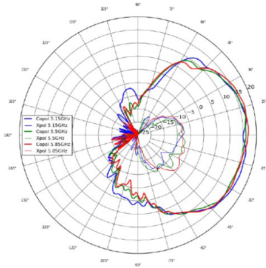
CH 6 Horizontal Polarization, Azimuth
