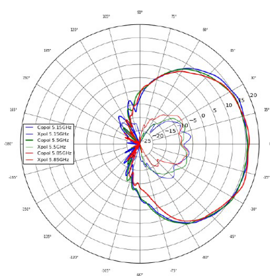
CH 5 Vertical Polarization, Azimuth
