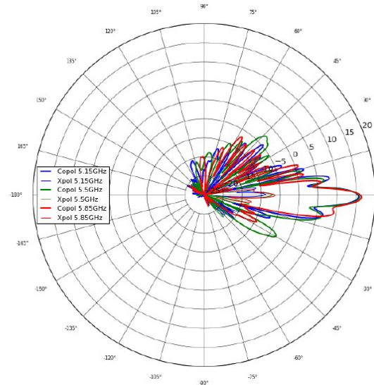
CH 2 Horizontal Polarization, Elevation
