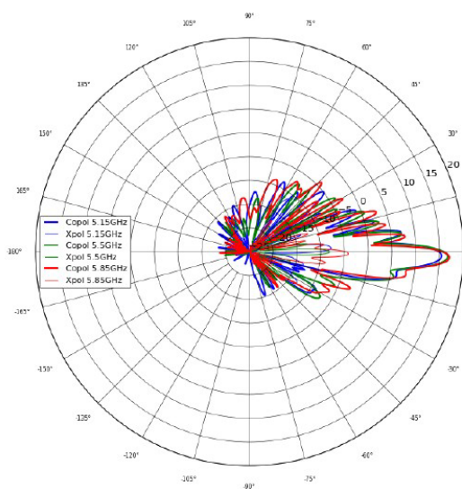
CH 0 Horizontal Polarization, Elevation
