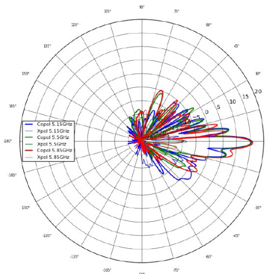
CH 3 Vertical Polarization, Elevation
